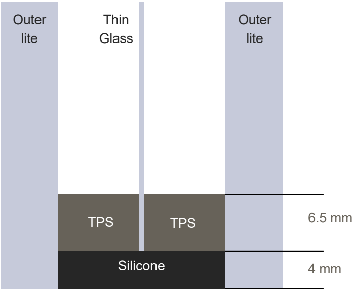
Figure 6. Sightline spec of TPS system to be used for thermal simulation purposes
