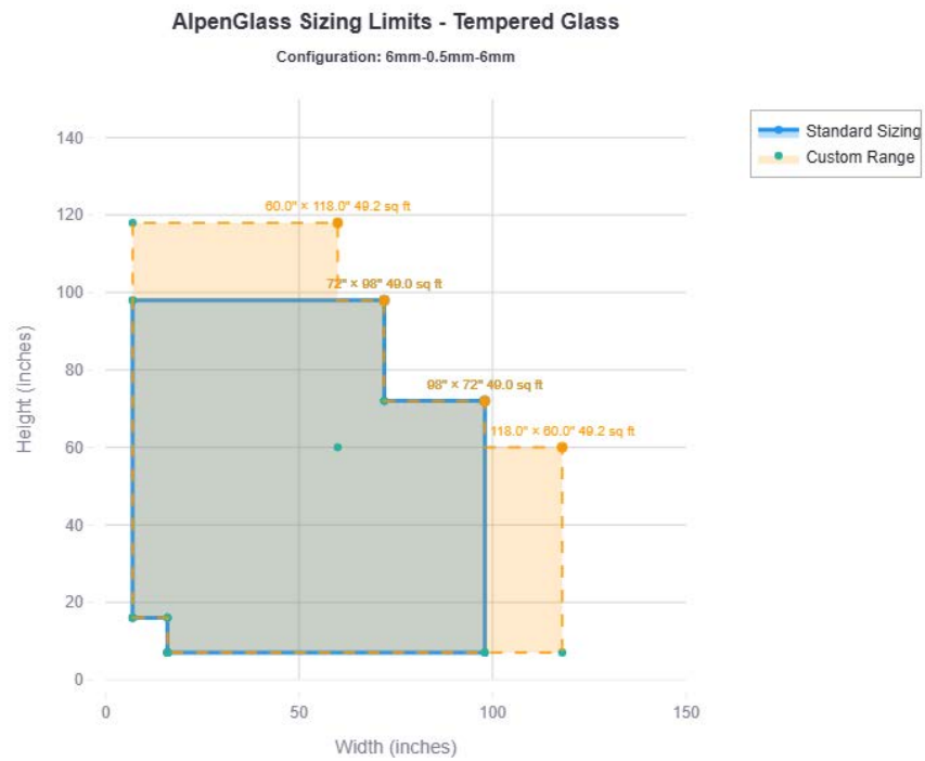
Figure 21. Tempered 6mm-0.5mm-6mm
