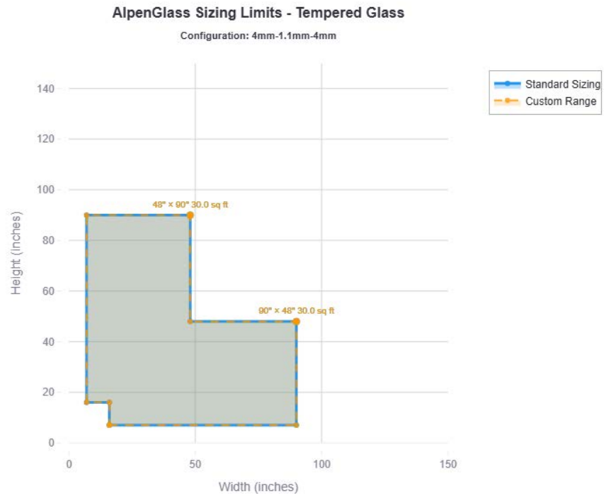
Figure 16. Tempered 4mm-1.1mm-4mm
