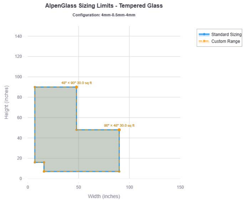
Figure 15. Tempered 4mm-0.5mm-4mm
