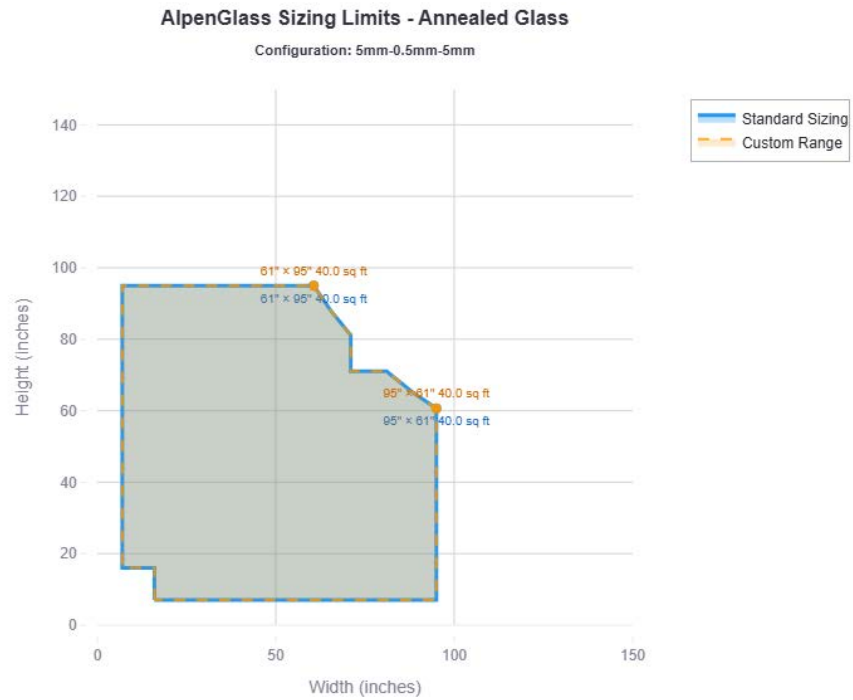
Figure 30. Annealed 5mm-0.5mm-5mm
