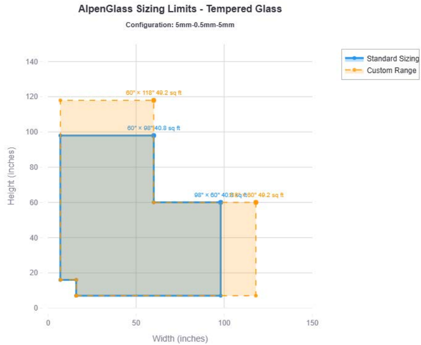
Figure 18. Tempered 5mm-0.5mm-5mm
