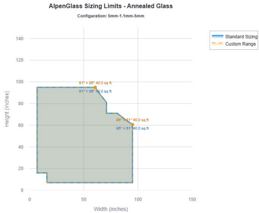
Figure 31. Annealed 5mm-1.1mm-5mm
