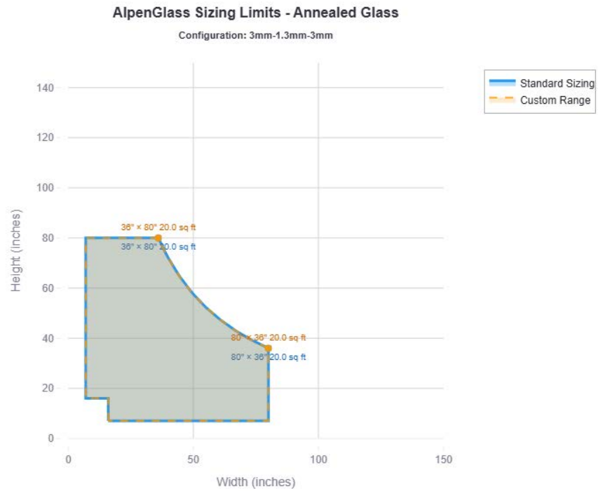
Figure 26. Annealed 3mm-1.3mm-3mm
