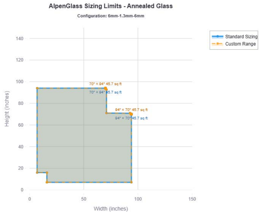
Figure 35. Annealed 6mm-1.3mm-6mm
