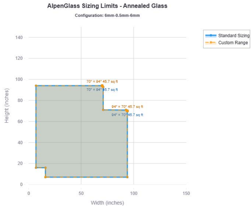
Figure 33. Annealed 6mm-0.5mm-6mm
