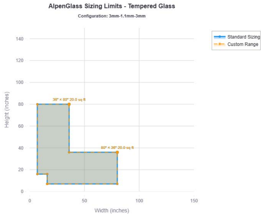
Figure 13. Tempered 3mm-1.1mm-3mm
