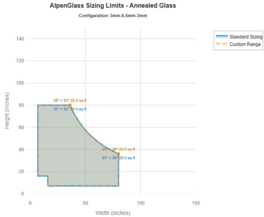
Figure 24. Annealed 3mm-0.5mm-3mm
