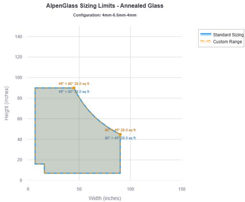
Figure 27. Annealed 4mm-0.5mm-4mm
