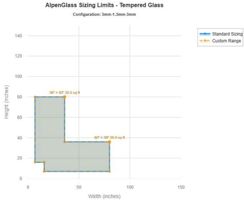
Figure 14. Tempered 3mm-1.3mm-3mm
