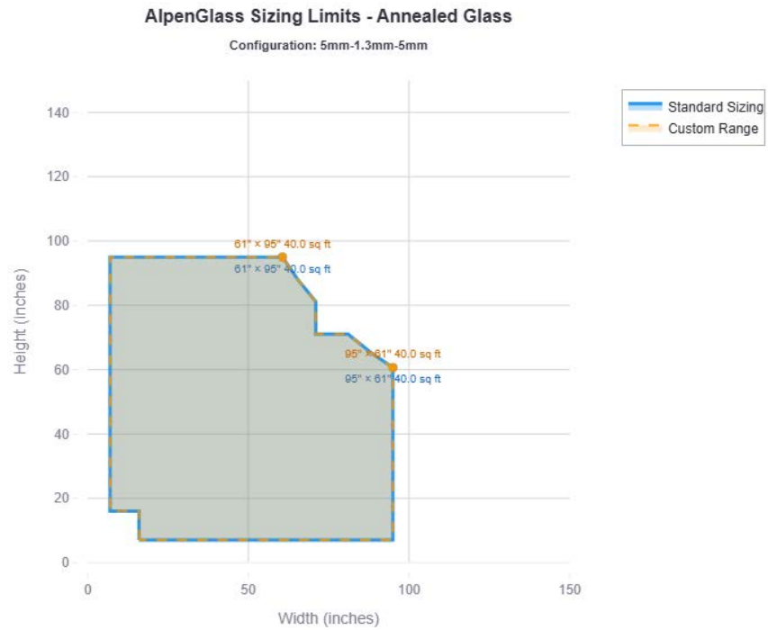
Figure 32. Annealed 5mm-1.3mm-5mm
