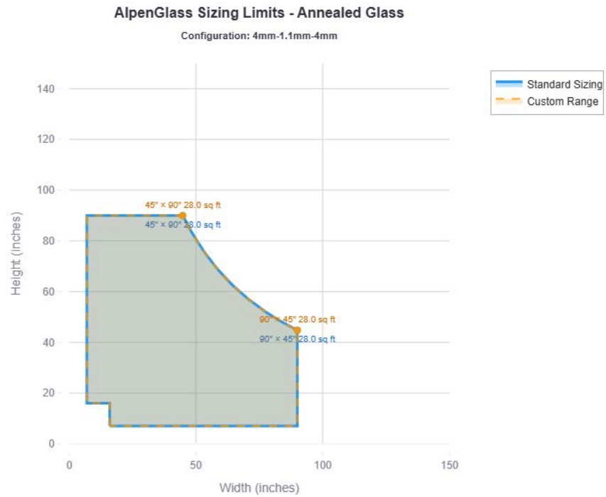
Figure 28. Annealed 4mm-1.1mm-4mm
