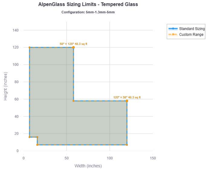
Figure 20. Tempered 5mm-1.3mm-5mm
