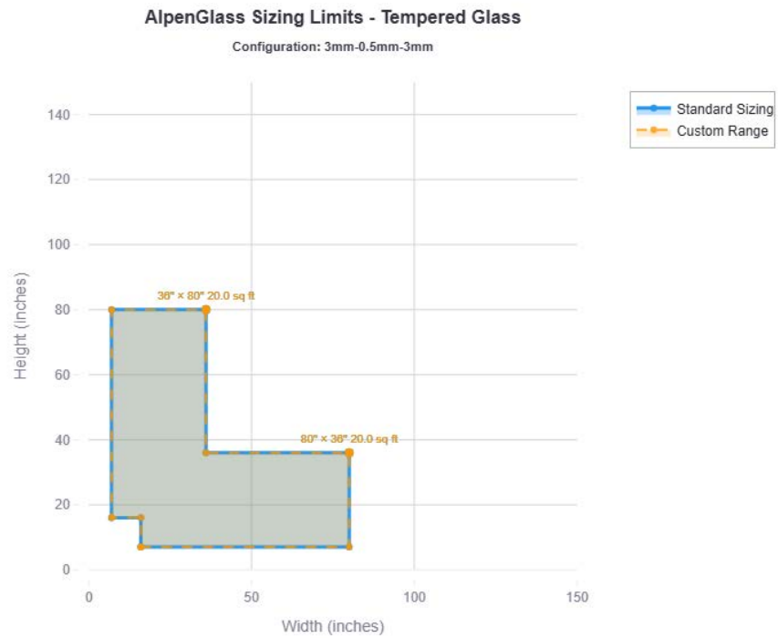
Figure 12. Tempered 3mm-0.5mm-3mm
