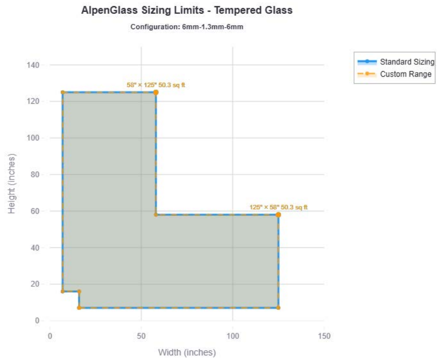
Figure 23. Tempered 6mm-1.3mm-6mm
