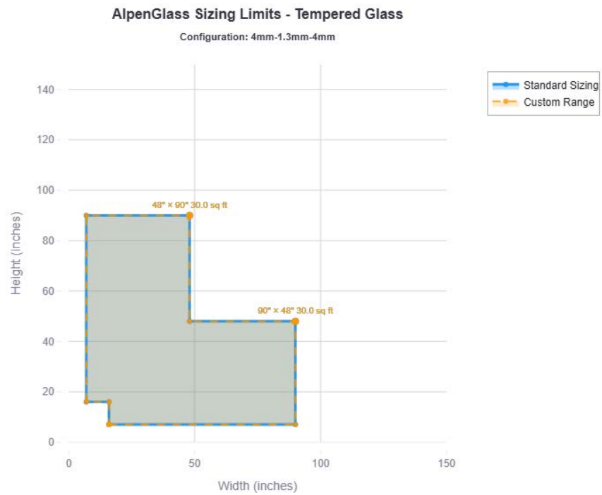
Figure 17. Tempered 4mm-1.3mm-4mm
