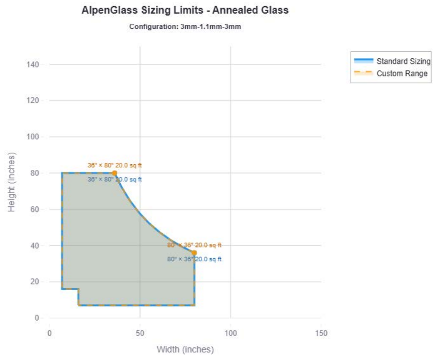
Figure 25. Annealed 3mm-1.1mm-3mm
