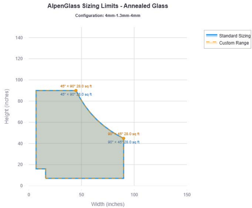
Figure 29. Annealed 4mm-1.3mm-4mm
