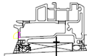
Single-hung example
