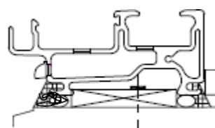
Double-hung example
