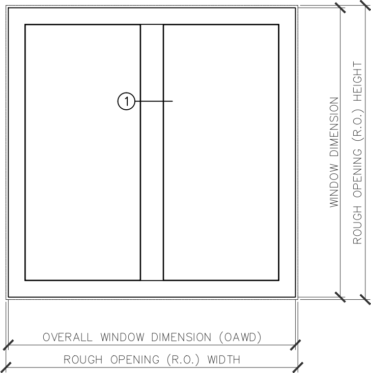
FIXED TO FIXED WINDOW SCALE 0'-3/4"=1'-0"
