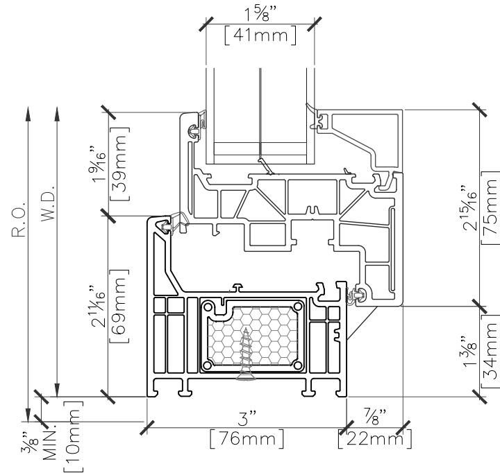
2 HOPPER WINDOW SECTION PROFILE @ SILL SCALE 6" = 1'-0"
