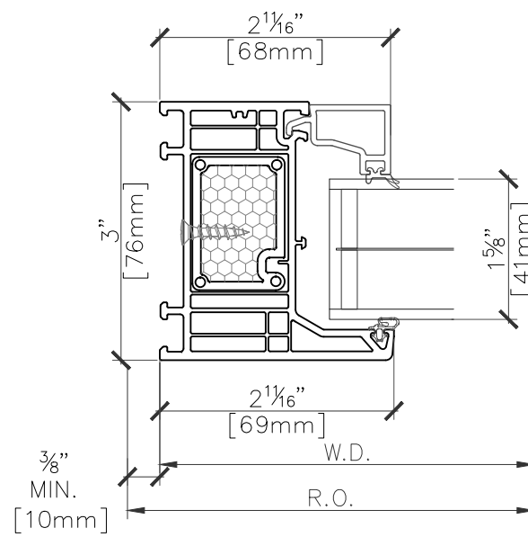
3 FIXED WINDOW SECTION PROFILE @ JAMB SCALE 6" = 1'-0"
