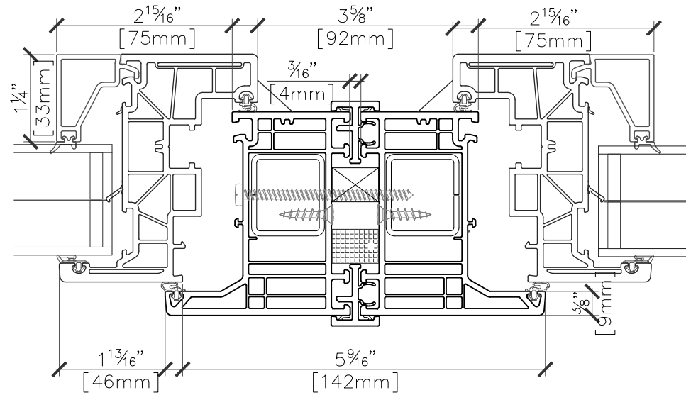
OPERABLE TO OPERABLE WINDOW SECTION PROFILE SCALE 6" = 1'-0"
