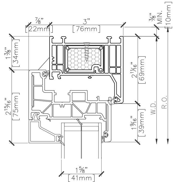
1 HOPPER WINDOW SECTION PROFILE @ HEAD SCALE 6" = 1'-0"
