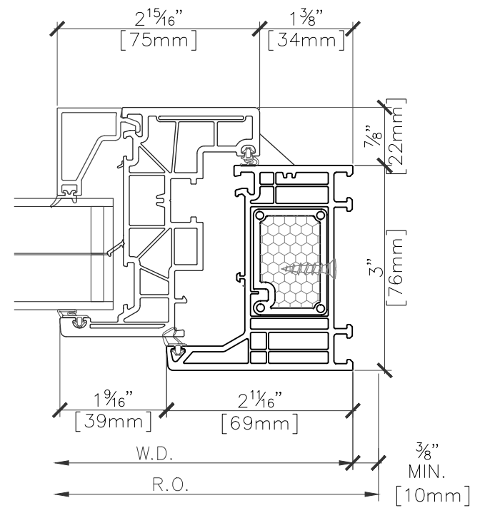
TILT-TURN WINDOW SCALE 0'-3/4"=1'-0"
