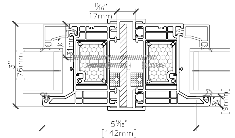
Combination Structural Mull 6371+3x76
