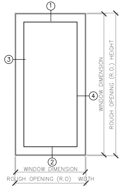
FIXED WINDOW SCALE 0'-3/4"=1'-0"
