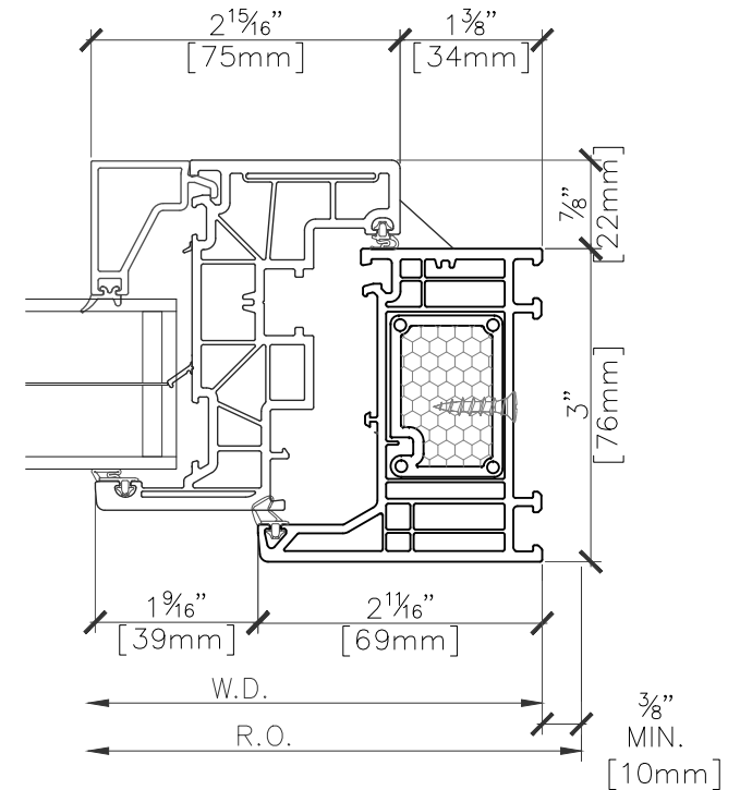
HOPPER WINDOW SCALE 0'-3/4"=1'-0"
