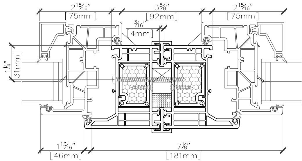
OPERABLE TO OPERABLE WINDOW SECTION PROFILE SCALE 6" = 1'-0"
