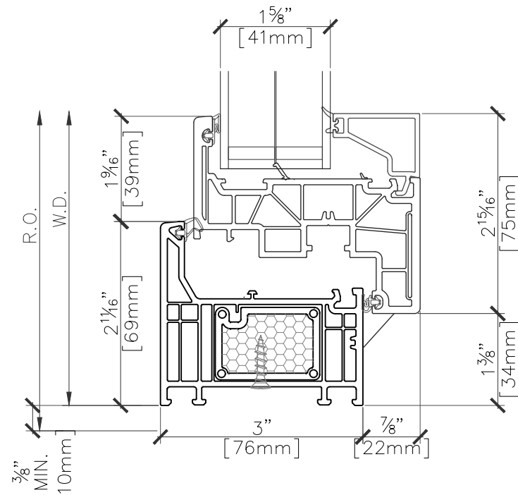
2 TILT-TURN WINDOW SECTION PROFILE • SILL SCALE 6" = 1'-0"
