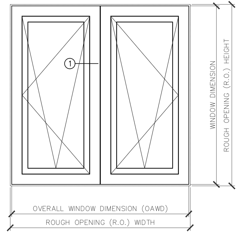
OPERABLE TO OPERABLE WINDOW SCALE 0'-3/4"=1'-0"
