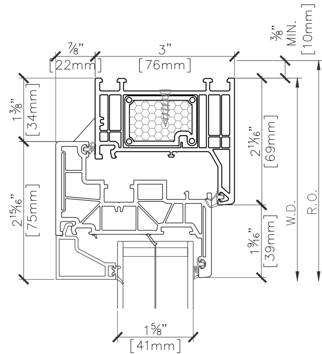
1 TILT-TURN WINDOW SECTION PROFILE • HEAD SCALE 6" = 1'-0"
