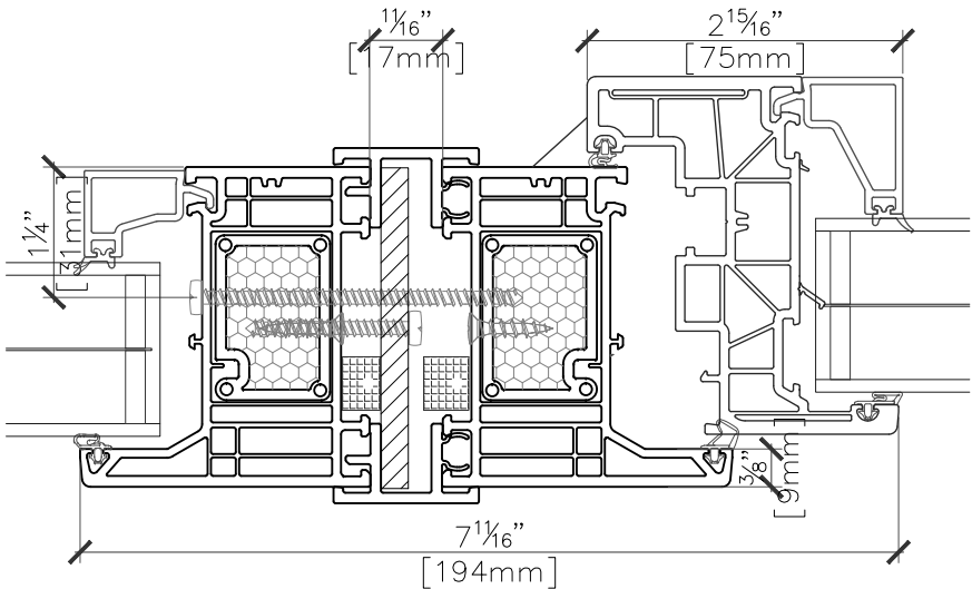
Combination Structural Mull 6371+3x76 [23 ]
