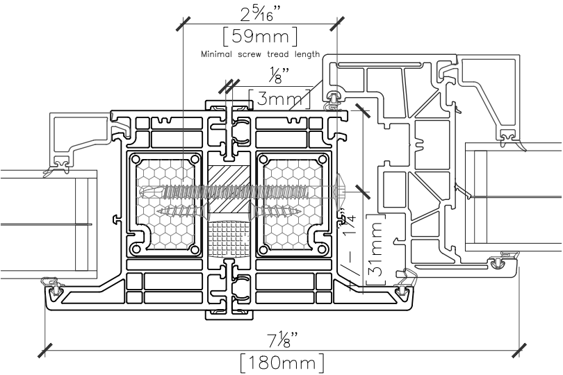
Combination Tight Mull 6370
