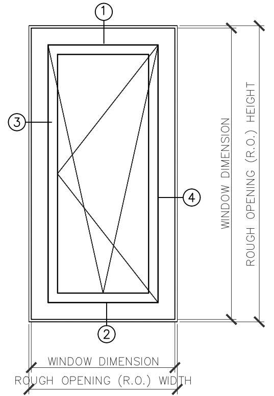
TILT-TURN WINDOW SCALE 0'-3/4"=1'-0"
