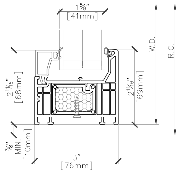
2 FIXED WINDOW SECTION PROFILE @ SILL SCALE 6" = 1'-0"
