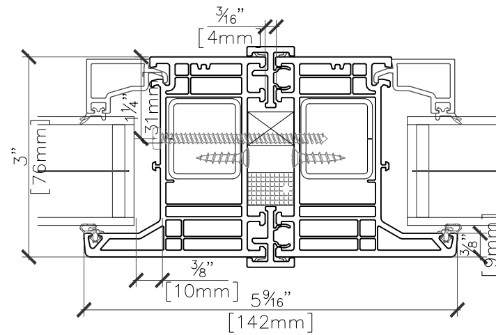
Combination Tight Mull 6370 | U-1675
