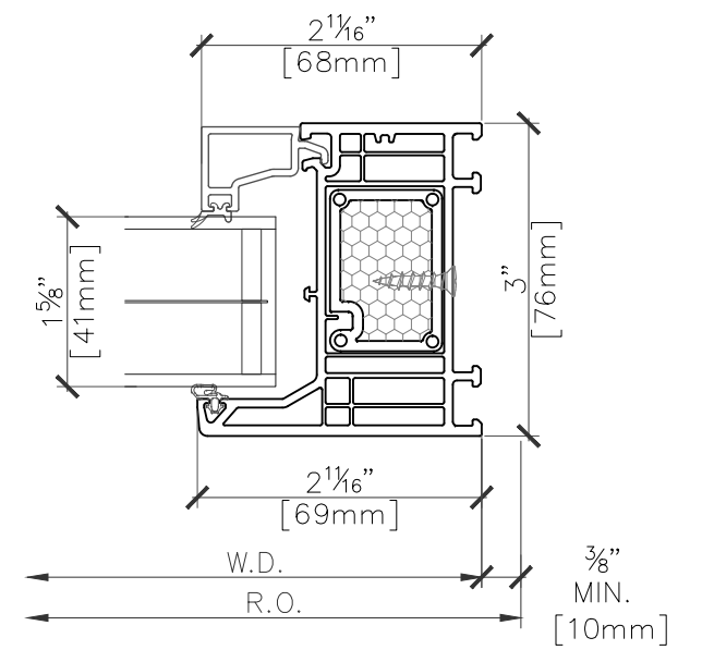
4 FIXED WINDOW SECTION PROFILE @ JAMB SCALE 6" = 1'-0"
