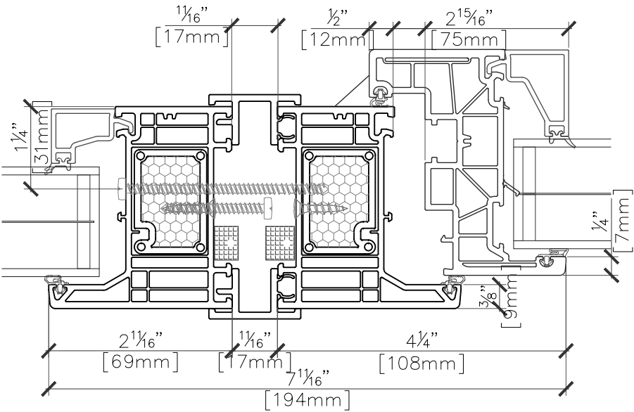
Combination Structural Mull 6371+9x76 [35.4]
