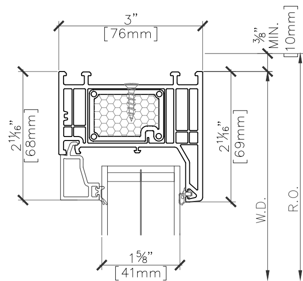
1 FIXED WINDOW SECTION PROFILE @ HEAD SCALE 6" = 1'-0"
