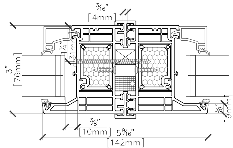
Combination Tight Mull 6370
