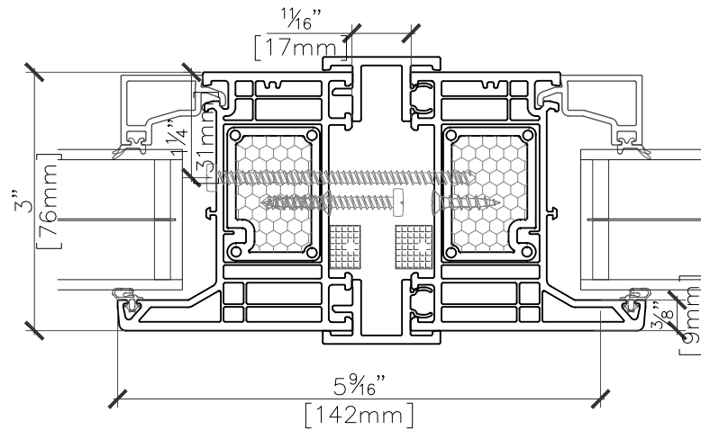
Combination Structural Mull 6371+9x76
