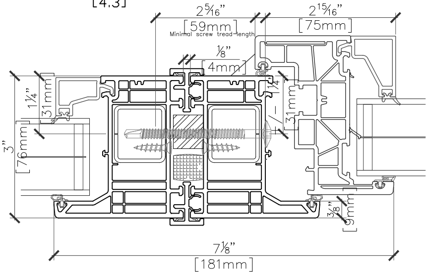
Combination Tight Mull 6370 | U-1675 [4.3]
